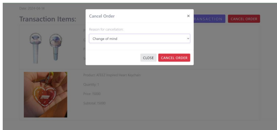
Gambar XV. Cancel Order 1.
