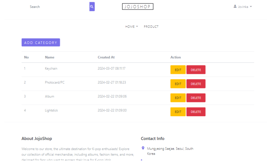
Gambar XIX. Halaman Category .
