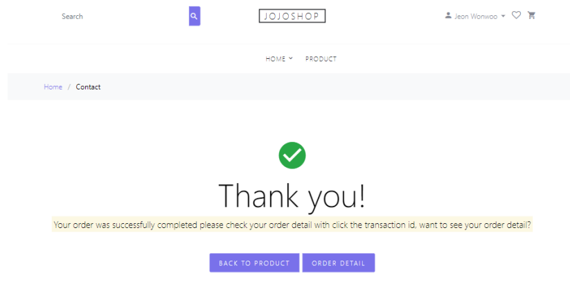
Gambar XI. Halaman Thankyou .
