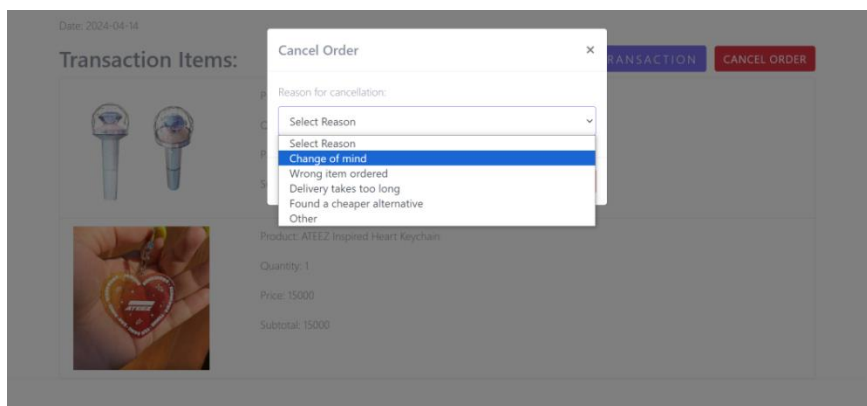
Gambar XVII. Cancel Order 3.
