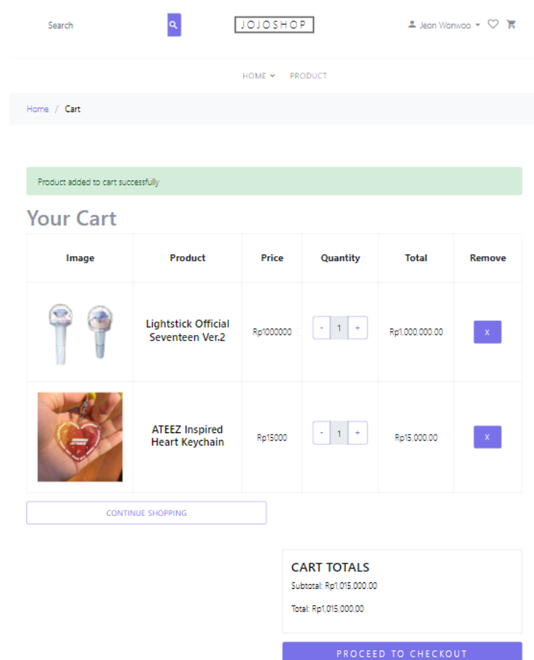
Gambar IX. Halaman Cart.
