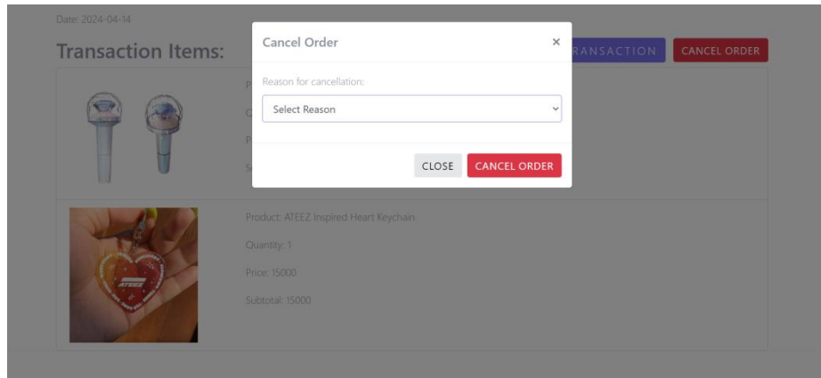
Gambar XV. Cancel Order 1.
