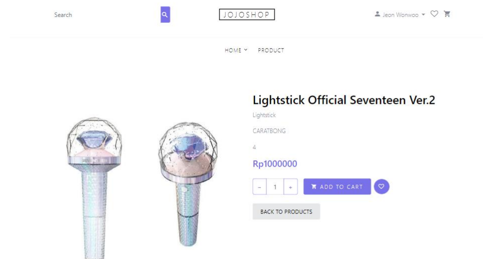
Gambar VII. Halaman View .
